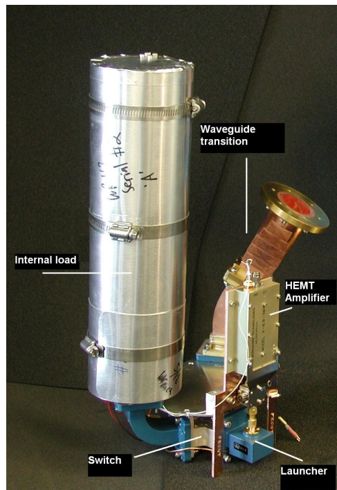
FIG. 8.— Photograph of cold stage of ARCADE 2 8 GHz radiometer. The throat of the horn antenna bolts to the open circular waveguide end. The internal reference load of this radiometer is a wedge termination in waveguide, which is surrounded by the insulative cylinder visible in the photograph.
