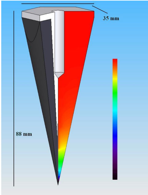
FIG. 9.— Cut away view of external calibrator cone showing internal structure and predicted linear temperature profile from the 2006 flight, with the base thermally fixed and the cone immersed in a cold atmosphere. The cone consists of Steelcast absorber (black) cast onto an aluminum core (light grey). There is also a copper wire running from the tip of the aluminum core to nearly the tip of the cone (darker grey). The hole in the base is threaded for a mounting bolt to affix the cone to the aluminum back plate. The measured thermal gradient is 600 mK from the base to the tip of the cones. 98% of the total gradient is in a region near the tip containing 3% of the absorber, and the mean depth for absorption varies with frequency.
